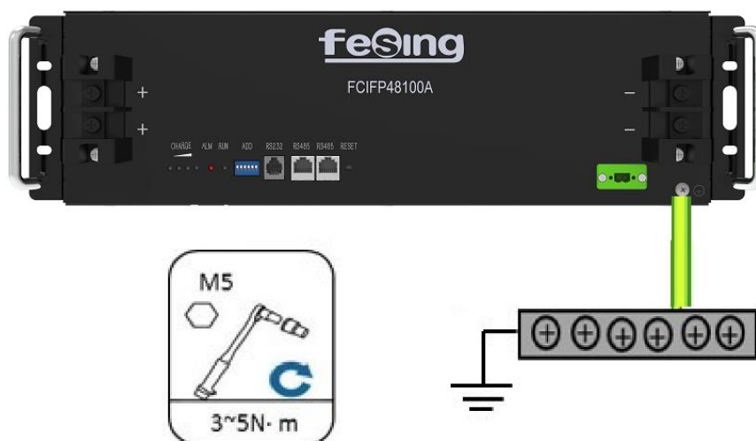
Figure 5-1: Install the Grounding Wire
