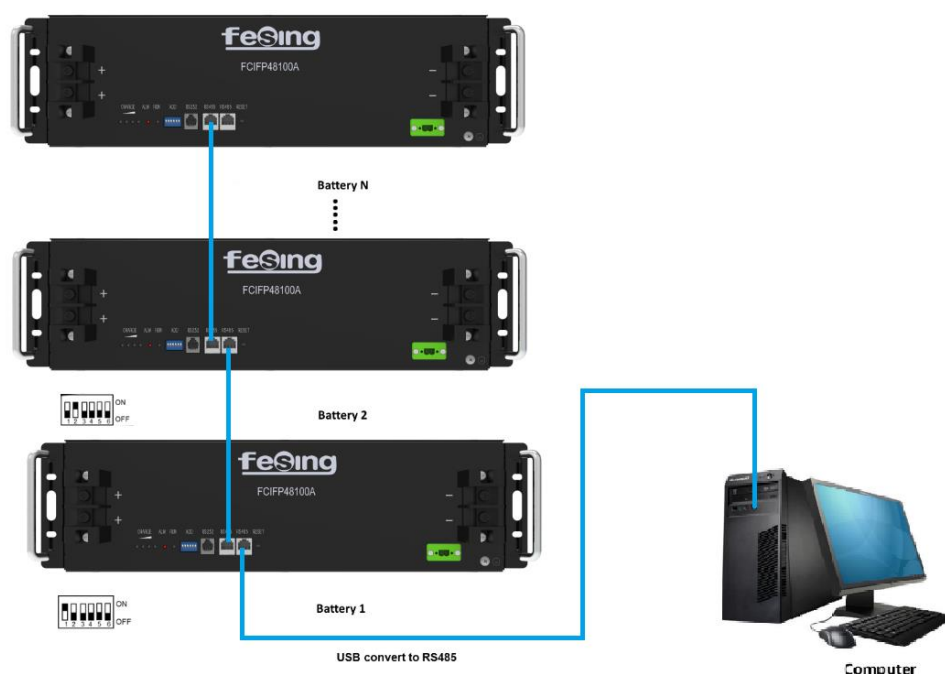
Figure 5-6: Communication Cable Connections among Multiple Batteries
