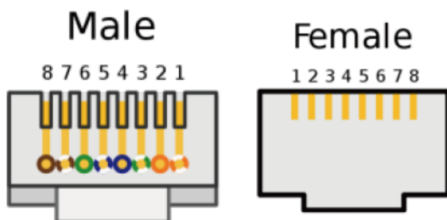
(a) RJ45 Pin Male
